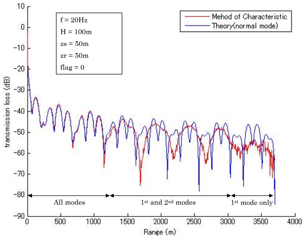
FIGURE Sample output of 2-D MC: Comparison of transmission loss. The group velocities of 1 st , 2 nd , and 3 rd modes excited are respectively 1473 m/s, 1240 m/s, and 522 m/s. The loss matches the theory in the range where all modes have propagated.
